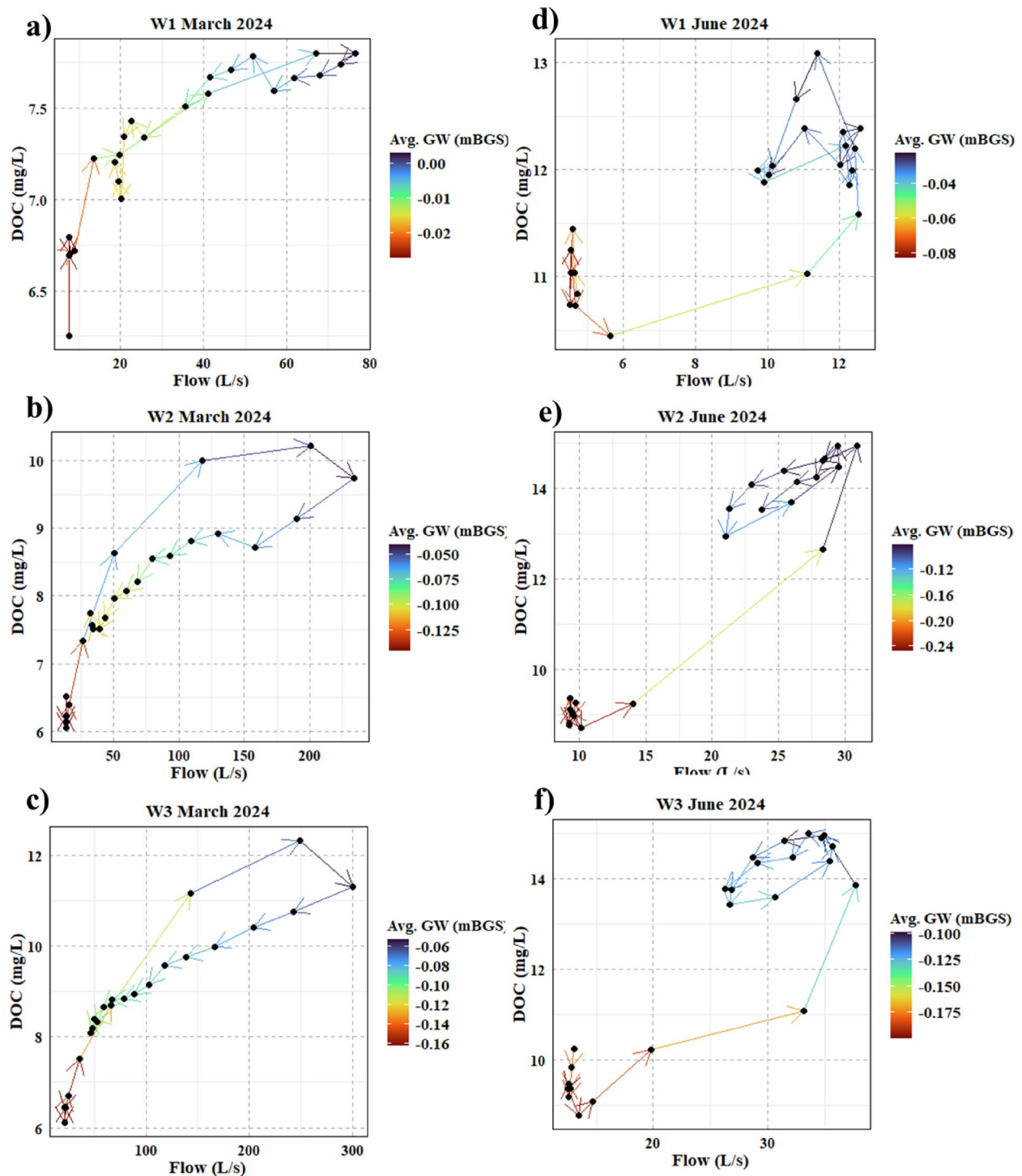
Fig. 7 Impact of seasonality and degradation on DOC variability and pathway of March 2024 (left) [(a), (b), (c)] and June 2024 (right) [(d), (e), (f)] event moving downstream from W1 (near-intact) to W3 (degraded)
