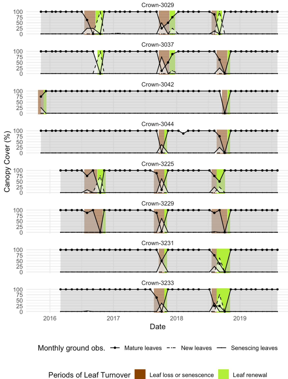
Figure 2. Ground observations of Moabi leaf turnover at Lopé NP, Gabon (2015–2019). The solid and dashed lines show the scores given for canopy coverage of mature, senescing, and new leaves at each monthly observation. The brown and green rectangles show the likely periods of either leaf senescence and loss (brown rectangles) or leaf renewal (green rectangles) based on the monthly observations as defined in Figure 1.
