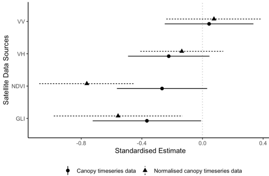
Figure 4. Detecting leaf senescence and loss using satellite data. Standardized estimates (dots) and 95% confidence intervals (lines) from eight single variate generalized linear mixed models (binomial) for the probability of detecting leaf senescence and loss from focal canopy time series (mean value of all pixels within canopy) and normalized canopy time series (difference between the mean value of all pixels within the canopy and the mean value of all pixels in the surrounding forest buffer) of the VV and VH bands of the Sentinel-1 synthetic aperture radar (SAR) data and the normalized difference vegetation index (NDVI) and the green leaf index (GLI) derived from Sentinel-2 optical data. Mixed models included tree ID and year as random effects.
