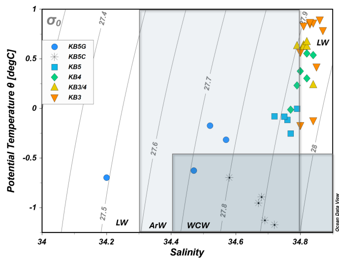
FIGURE 2 Temperature and salinity plot for all depths (0–300 m) to identify water masses in Kongsfjorden during spring. The masses identified were Local Water (LW), Arctic Water (ArW), and Winter Cooled Water (WCW). Water masses were calculated following Svendsen et al. (2002) and Cottier et al. (2005).
