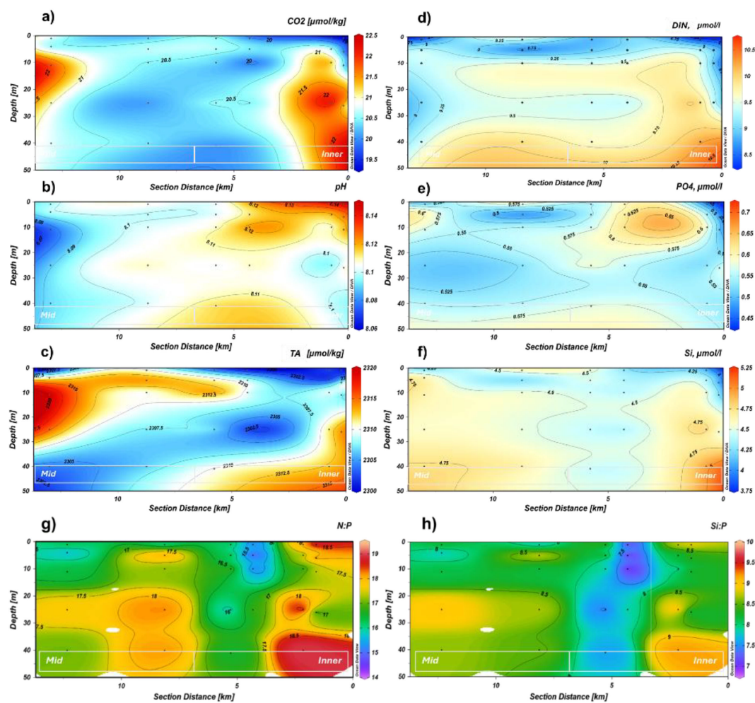
FIGURE 6 Profile section of the marine transect for (a) \text{CO}_2 , (b) pH, (c) TA, (d) DIN, (e) \text{PO}_4 , (f) Si, (g) N:P and (h) Si:P in the upper 50 m.
