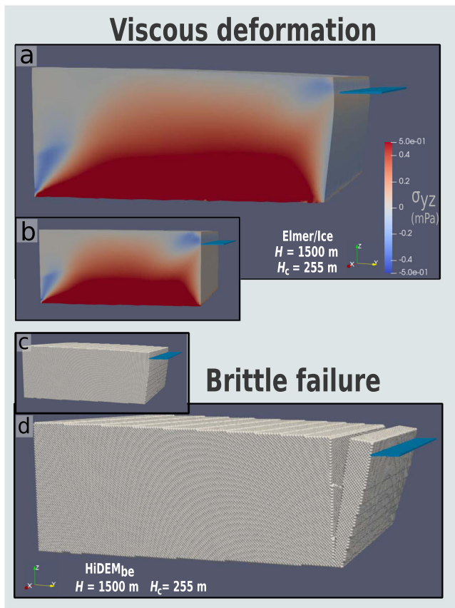
Fig. 1 Mode of structural failure in which tensile failure follows viscous deformation. a Viscous deformation of a glacier geometry as modeled in Elmer/Ice. The Cauchy shear stress tensor component aligned with flow direction ( \sigma_{yz} ) shows a maximum at the base and waterline of the calving face. b The geometry and \sigma_{yz} field shown in (a) prior to viscous deformation. c The brittle-elastic version of the Helsinki Discrete Element Model (HiDEM be ) domain initialized with the output geometry of the Elmer/Ice simulation in a . d An example of brittle failure in HiDEM be caused by tensile stress at the glacier surface leading to surface crevassing and calving via forward block rotation. H = calving face thickness; H_c = ice-cliff height.
