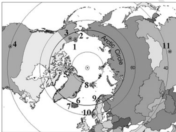
21 Fig. 6 ITEX sites contributing to the Walker et al. (2006) meta-analysis of plant community responses to experimental warming. (From Walker et al. 2006; reprinted with permission from the authors and Macmillan Magazines.)
