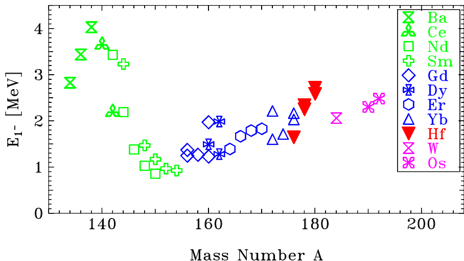
Fig. 1 Systematics of the excitation energy E_{1-} of the first excited 1_1^- level in the lanthanide/rare-earth region. Figure is taken from Ref. [19].
