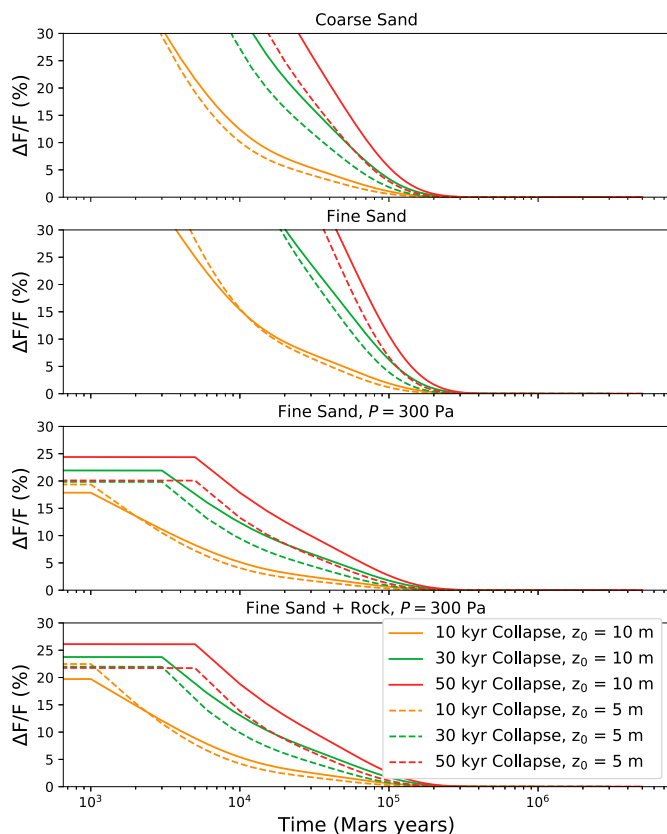
Fig. 4. Heat-flow perturbations, with time since the end of an atmospheric collapse, expected at 5 m depth (solid: z_0 = 10 m, dashed: z_0 = 5 m). The scenarios are, from top: collapse to 30 Pa with coarse-grained regolith, collapse to 30 Pa with fine-grained regolith, collapse to 300 Pa with fine-grained regolith, and collapse to 300 Pa with fine-grained regolith overlaying bedrock.
