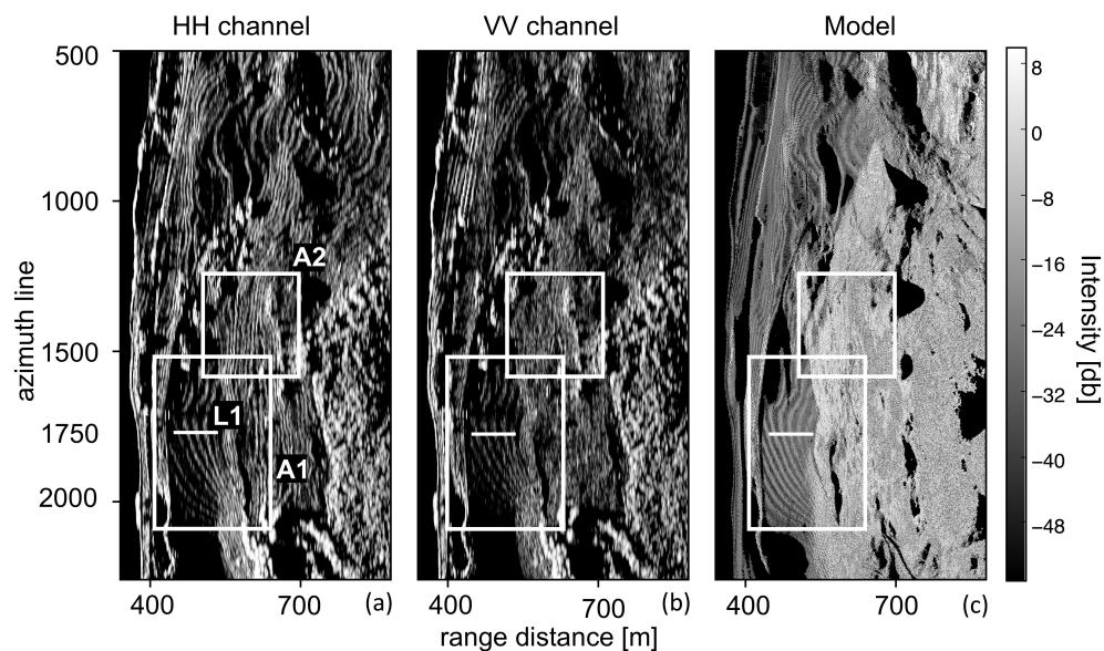
Figure 5. Radar backscatter images showing an MPI pattern at the Dorfberg test site in (a) horizontal and (b) vertical polarisation compared with (c) the modelled MPI. Area A1 highlights an area with a strong, low frequency MPI signal that are well visible in both polarisations and the model. Area A2 shows a higher frequency signal due to a steeper slope that are visible in the backscatter intensity image of the horizontal wave polarisation but hard to discern in the vertical polarisation and not present in the model. The white line corresponds to the central azimuth line used for the computation shown in Figure 6.
