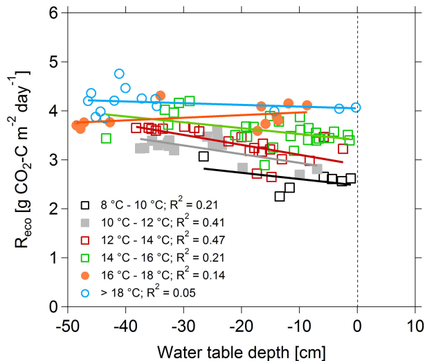
Figure 8. Ecosystem respiration as a function of water table depth and air temperature (daily means for May–September 2013).
