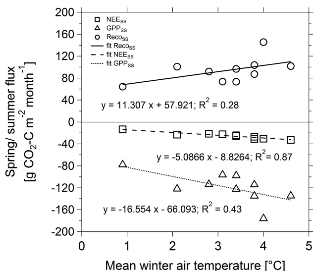
Figure 6. Spring/summer fluxes of NEE, GPP and R_{\text{eco}} (mean from April to September) as a function of the preceding winter's mean air temperature (mean from December to March).
