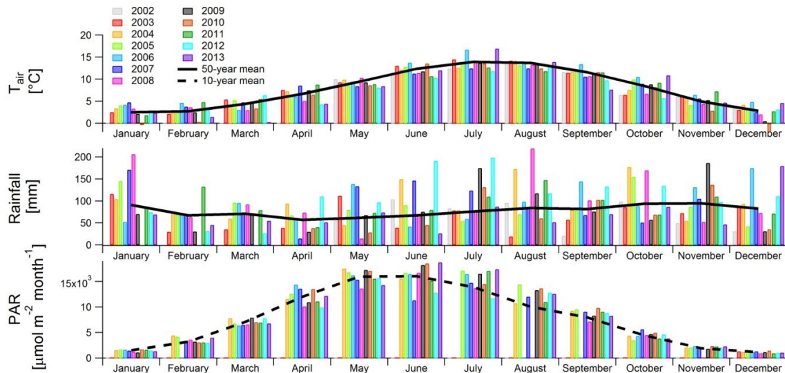
Figure 1. Monthly air temperature, rainfall and photosynthetically active radiation (PAR) for the study period 2002–2013.
