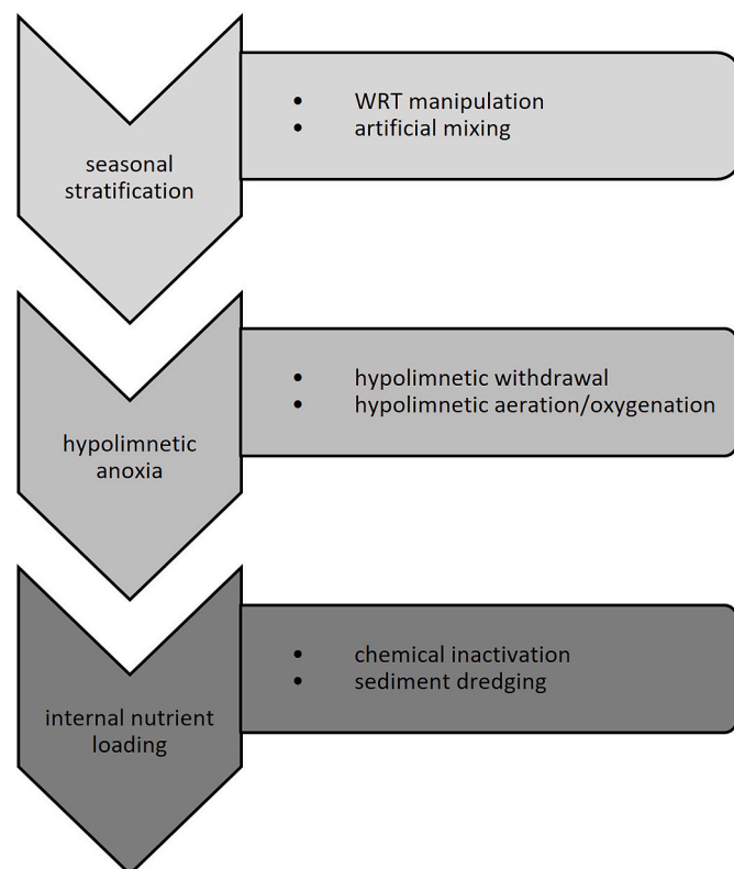
Fig. 1. Different aspects of the stratification → anoxia → internal P loading sequence are targeted by different in-lake restoration methods.
