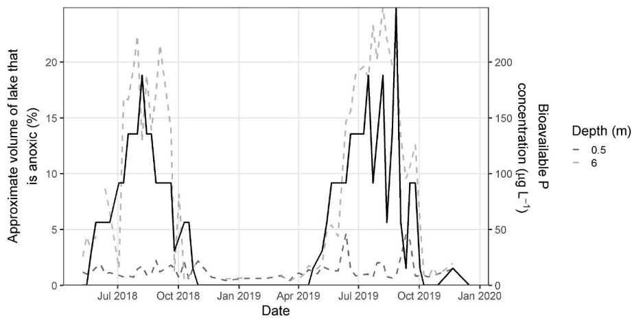
Fig. 6. Approximate volume of Elterwater-IB that is anoxic ( < 2 \text{ mg L}^{-1} , solid line) and concentration of biological available phosphorus (dashed lines) in the surface (0.5 m) and hypolimnion (6 m) based on profiles collected from May 2018 - December 2019.
