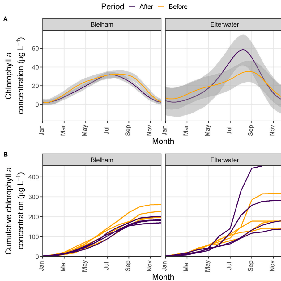
Fig. 5. a) average annual chlorophyll a dynamics (shading shows \pm 1 SE) and b) cumulative chlorophyll accumulation for each year before and after restoration at the control (Blelham) and impact (Elterwater-inner basin) lakes.
