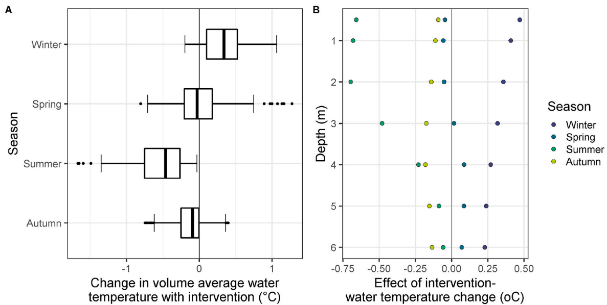
Fig. 3. a) change in volume averaged water column temperature in each season, b) water temperature changes at different depths with the intervention. Positive values indicate warming and negative values cooling, compared to water temperatures without the intervention.
