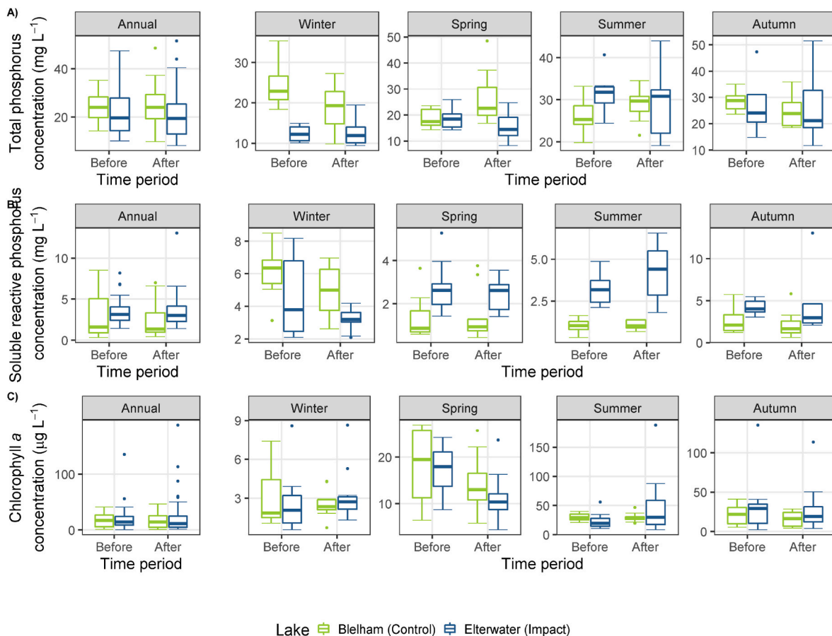
Fig. 4. a) Total phosphorus, b) soluble reactive phosphorus and c) chlorophyll a concentrations in Elterwater-IB (impact) and Blelham (control) sites before and after intervention, annually and grouped by season.
