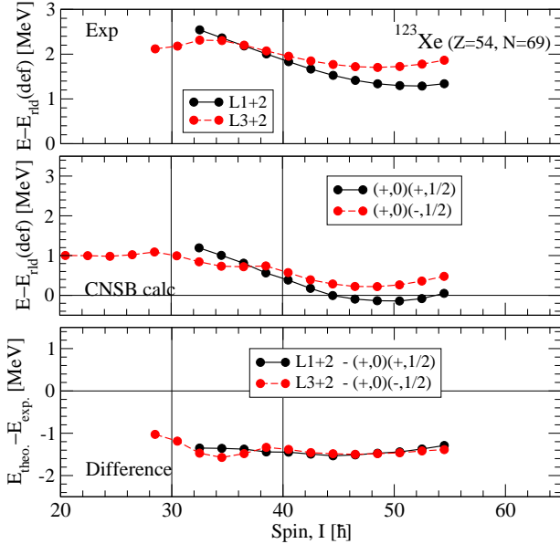
FIG. 10: (Color online) Comparisons between the observed bands L1 and L3 and the CNSB configurations assigned to them according to the comparison with CNS configurations, see Figs. 8 and 9.
