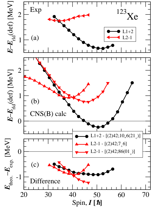
FIG. 9: (Color online) Same as Fig. 8 but for the L1 and L2 bands.
