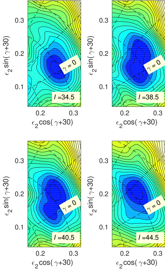
FIG. 11: (Color online) Total energy surfaces calculated in the CNSB formalism with constraints of parity and signature for protons and neutrons, (\pi, \alpha)_p(\pi, \alpha)_n = (+, 0)(-, 1/2) . This is the configuration assigned to the L3 band. The contour line separation is 0.2 MeV.
