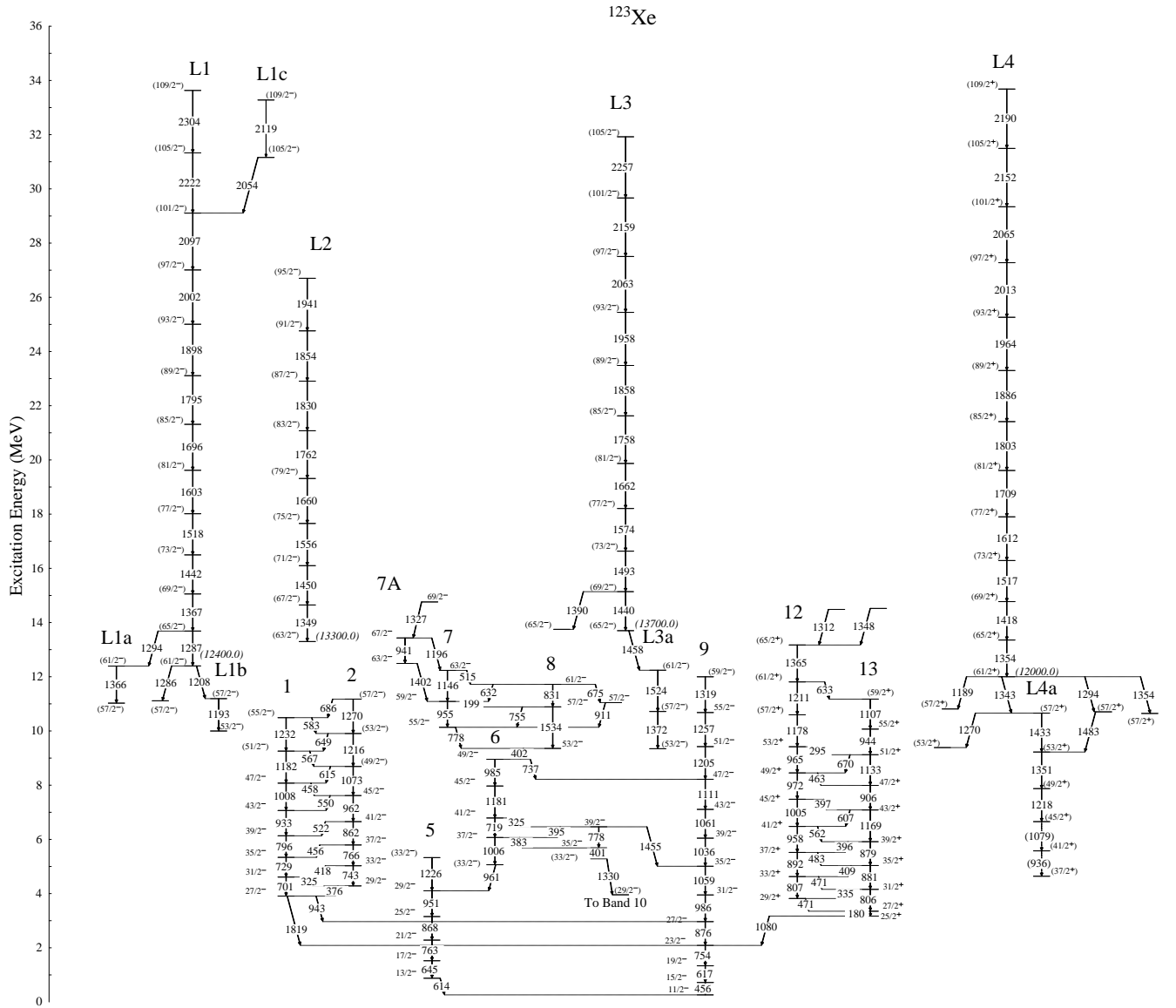
FIG. 1: Partial level scheme of ^{123}\text{Xe} showing the new high-spin bands L1-L4 described in the present work. The tentative level energies and spins of L1-L4 have been estimated from the patterns of their decays to ND levels (see text for details). The low-lying structures, numbered 1 to 13, are taken from Ref. [20].
