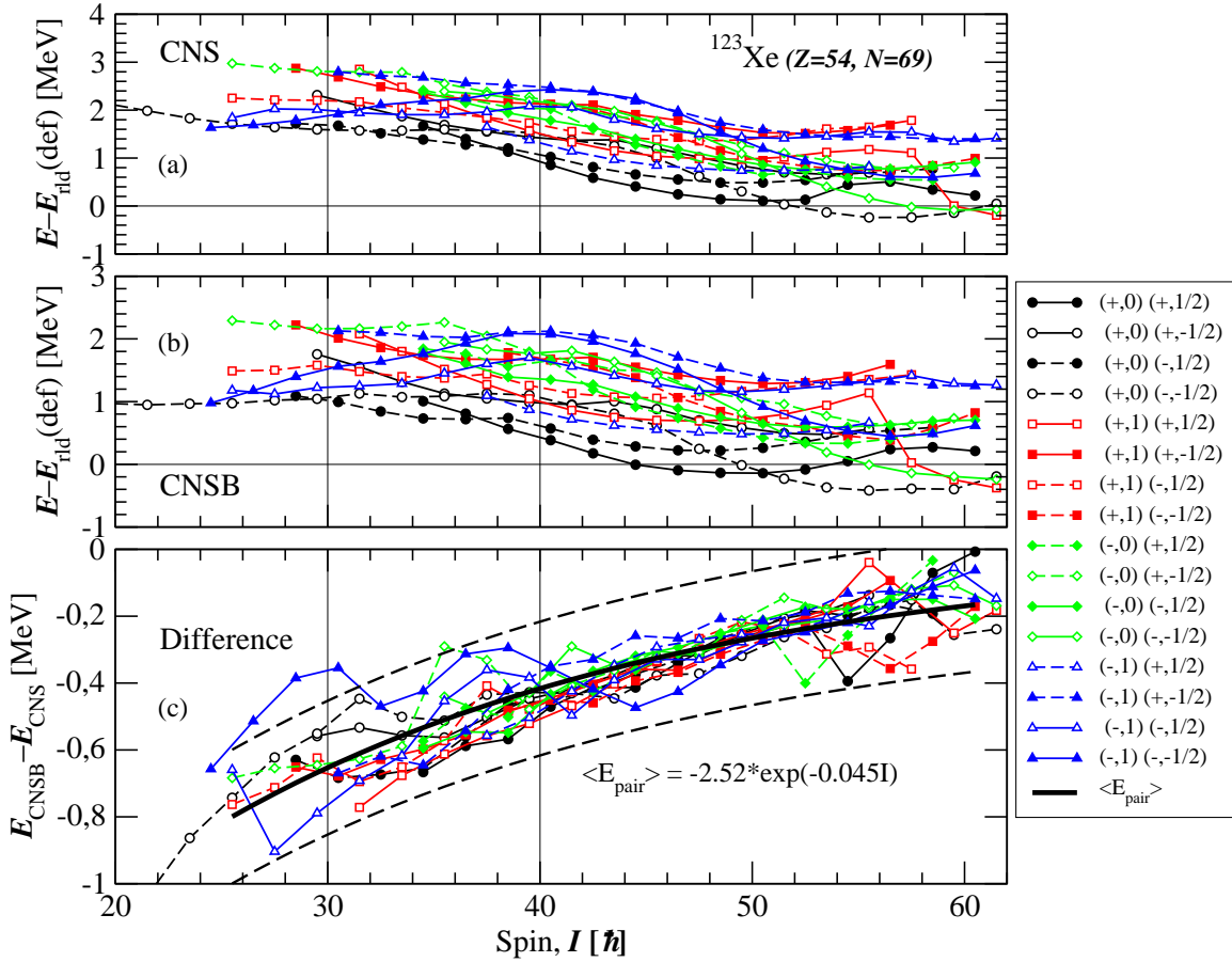
FIG. 5: (Color online) The energy of the minimum at \varepsilon_2 \approx 0.3 and a small \gamma deformation is shown relative to the rotating liquid drop model as calculated in the CNS model (a) and the CNSB model (b) for the 16 configurations with fixed parity and signature for protons and neutrons. The difference between these two calculations is presented in panel (c) where it is fitted to an exponential function labelled \langle E_{\text{pair}} \rangle . Note the expanded scale in the lower panel, where dashed lines illustrate the fact that almost all differences are fitted with an accuracy better than \pm 0.2 MeV.
