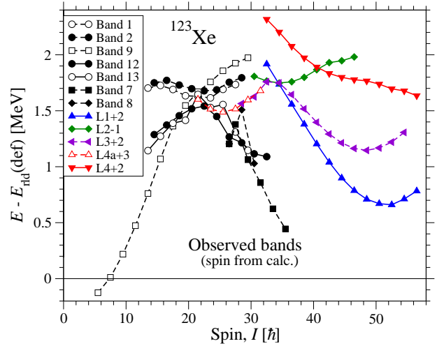
FIG. 12: (Color online) The observed collective bands in ^{123}\text{Xe} with spin values and excitation energies chosen from the comparison with calculated configurations are shown relative to the rotating liquid drop reference. In addition, some selected normal-deformed bands [20] are included.
